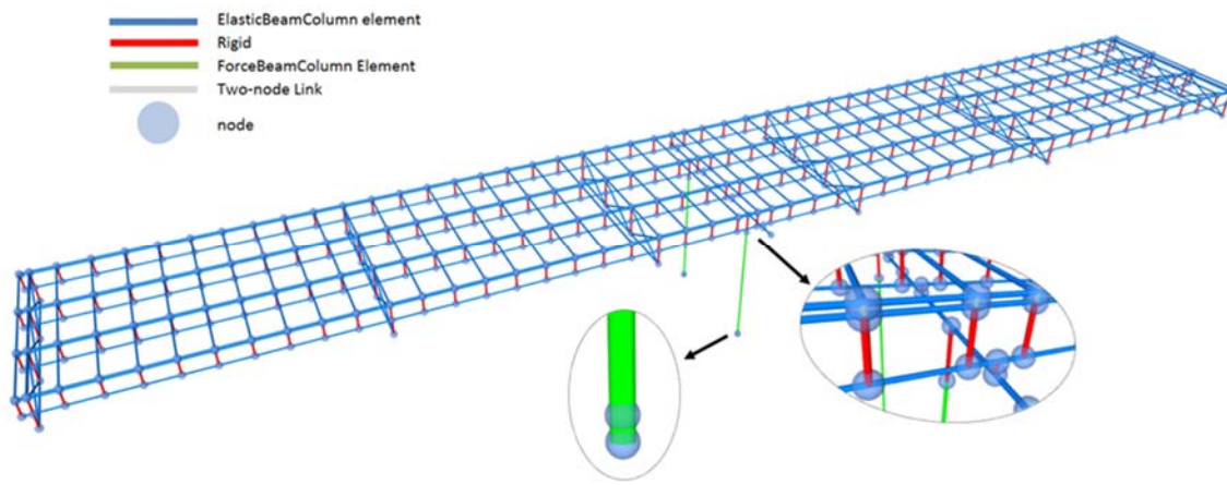
Fig. 1 – Detail of the superstructure elements and connection to the pier
