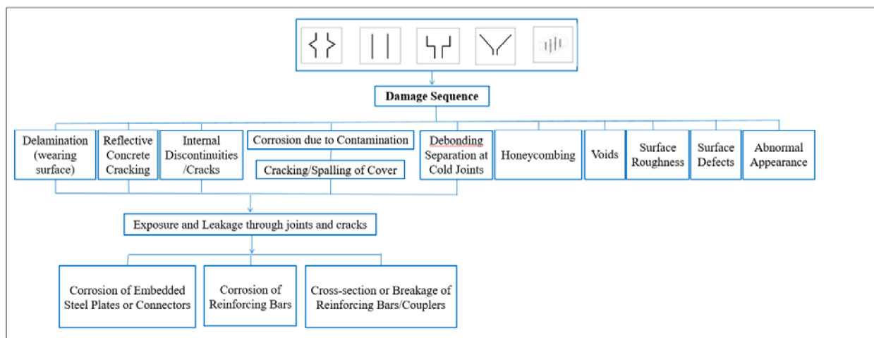
Figure 8: Sequence of damages for ABC closure joints [46-47]
