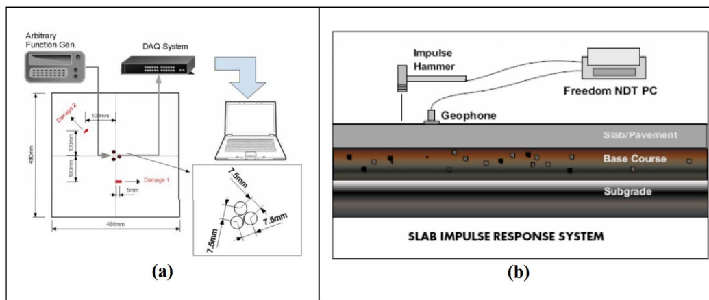
Figure 8: Examples of NDT test set-up. (a) Test set-up of PAU [37] (b) IRT application [39].
