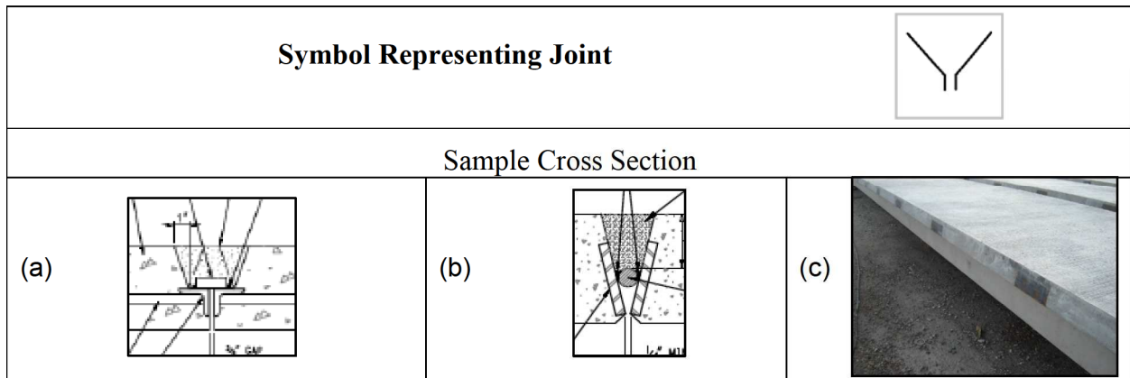
Figure 6: Type 4 Joint [7], [8], [12]
