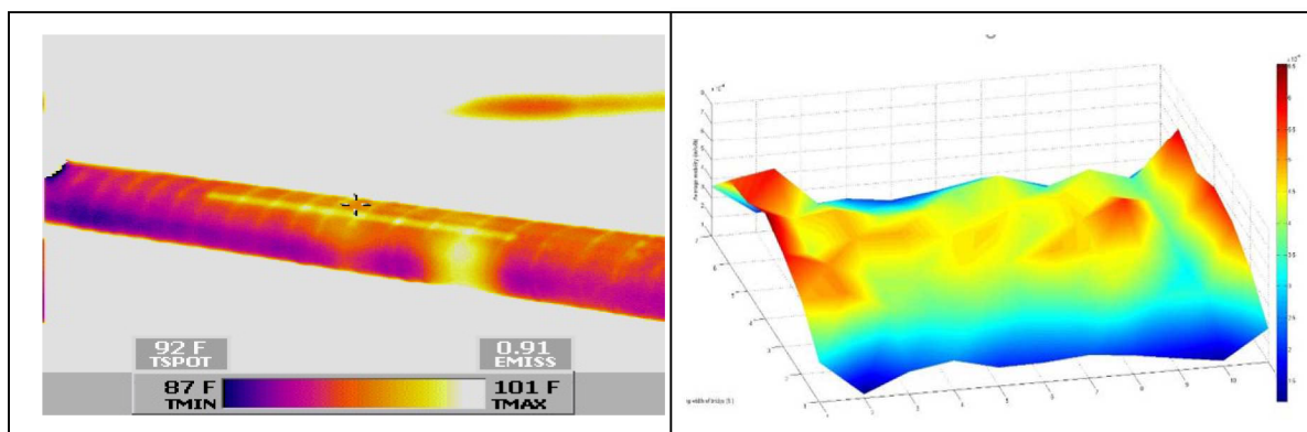
Figure 9: Examples of NDT results. (left) Infrared thermography image [38], (right) IRT result [45].
