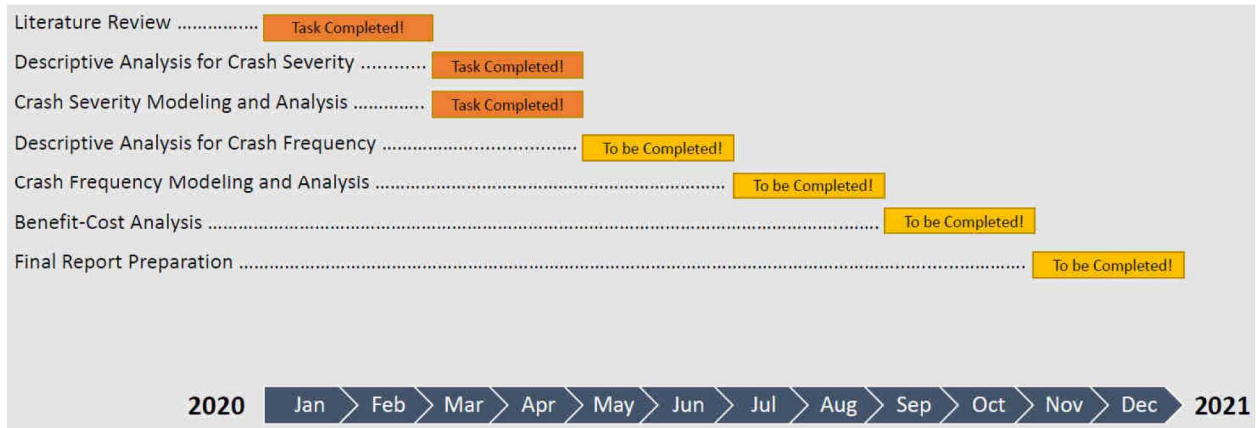
Figure 2: Project flowchart.
