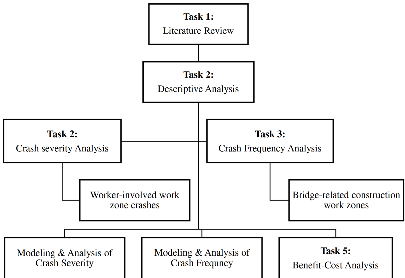
Figure 1: Project flowchart.
