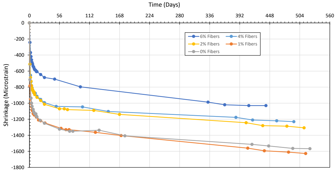
Figure 9. Shrinkage for each fiber content measured using ASTM C157
