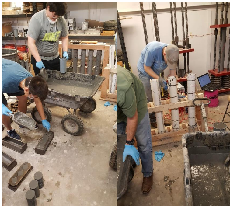
Figure 2. Casting of compression, shrinkage, and modulus of rupture test specimens (left) and creep specimens (right) for the 6% fiber mix
