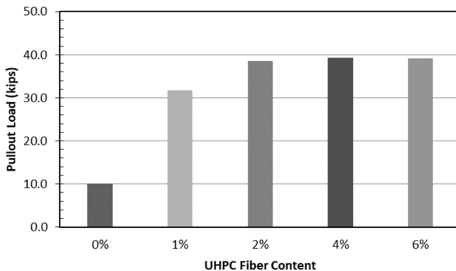
Figure 18. Pullout loads for No. 8 bar specimens with all fiber contents tested
