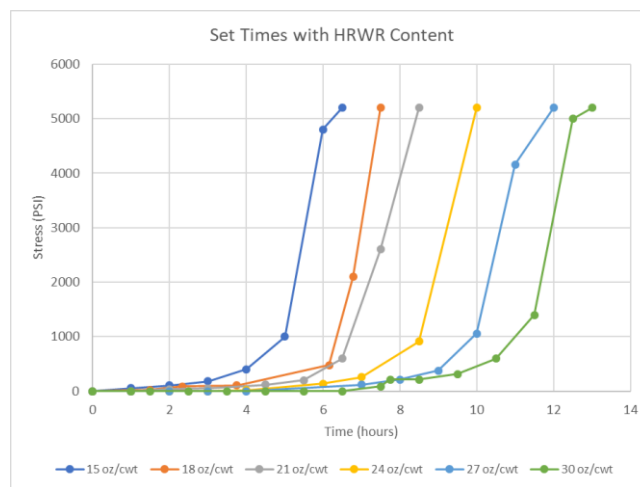
Figure 10. Results of ASTM C403 tests for set time with varying superplasticizer dosage
