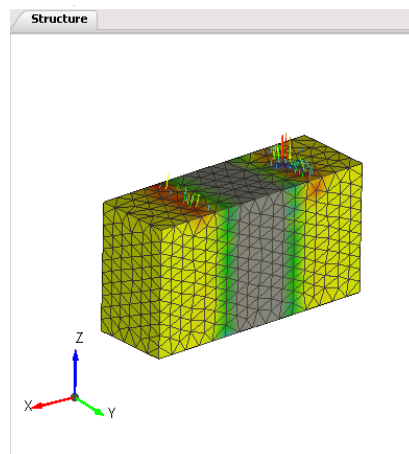
Figure 17. Numerical model of push-off tests using ATENA software.
