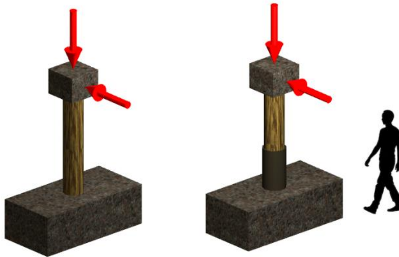
Figure 16. Test setup for large scale testing. (a) benchmark specimen for timber pile, (b) repaired timber pile with UHPC enhancement.
