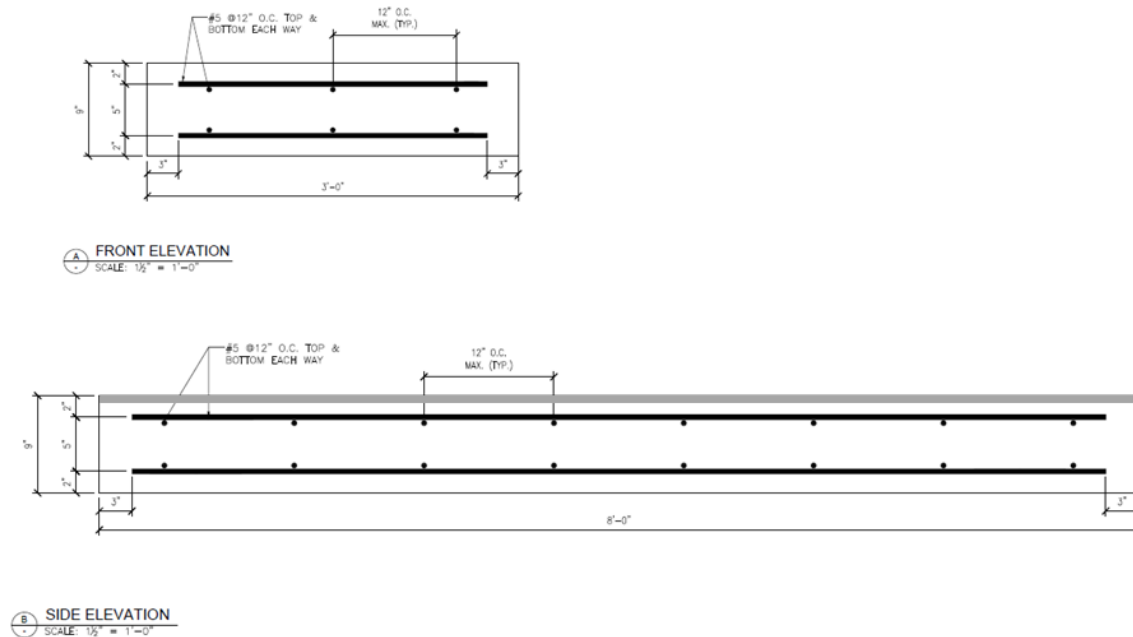
Figure 18. Details of the second specimen (Bridge Overlay)
