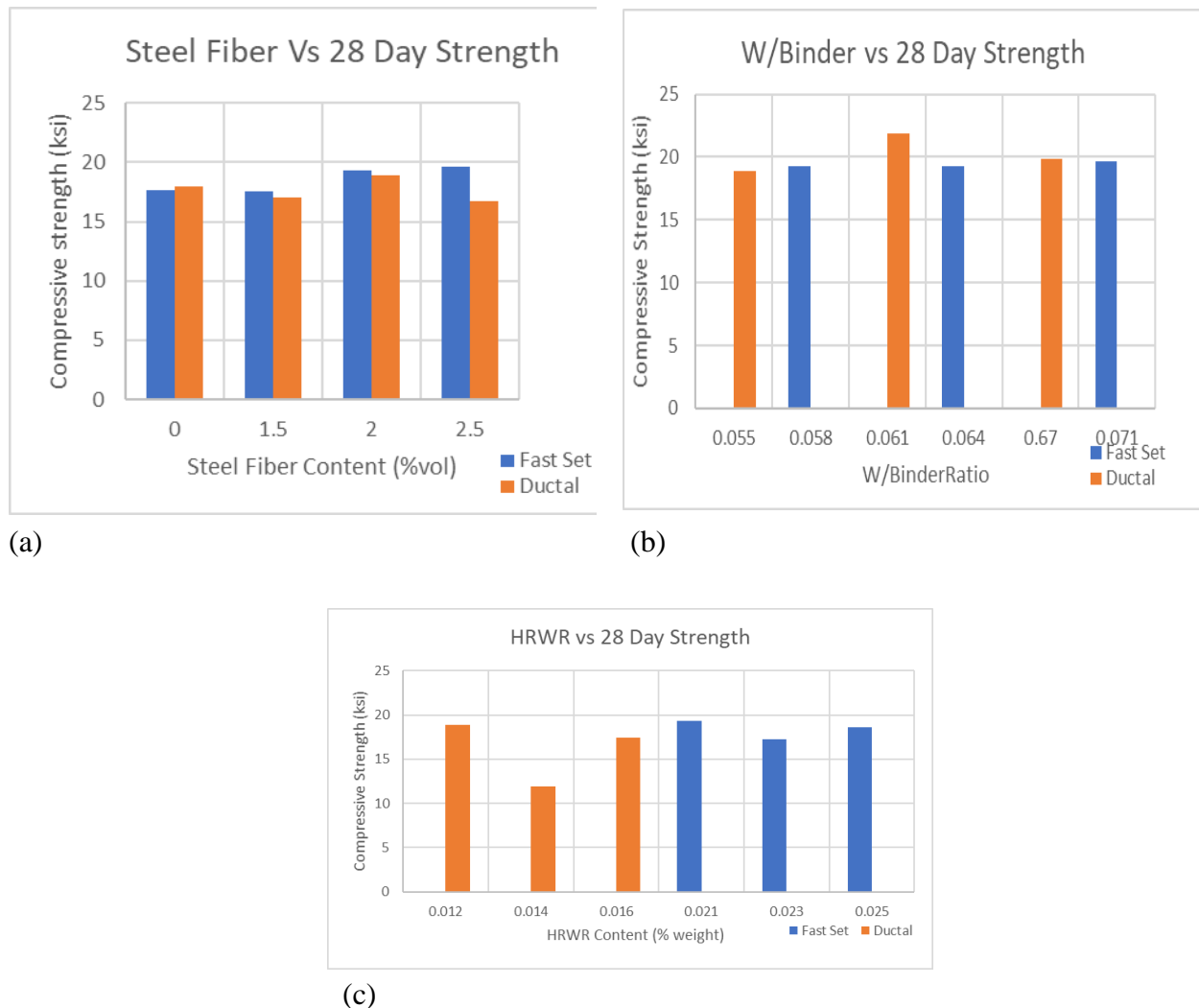
Figure 7. Compressive Strength Test Results
