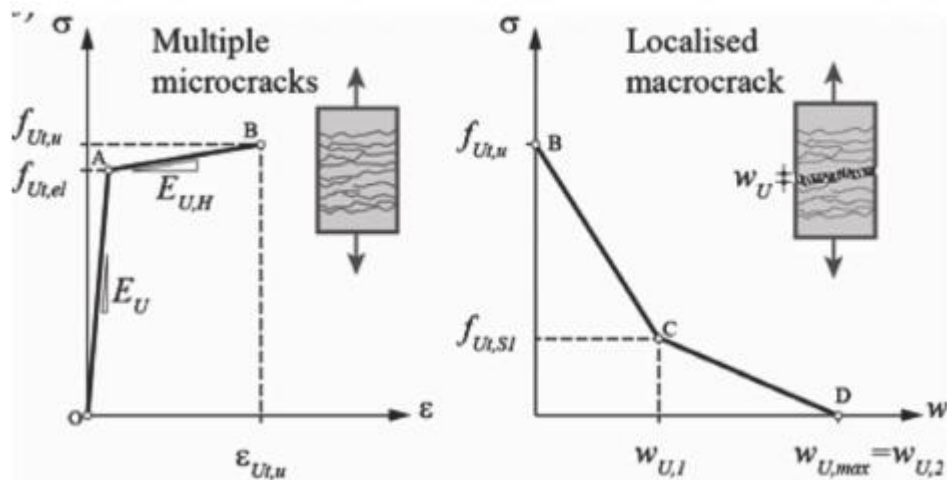
Figure 4. UHPC Tensile Behavior [10].
