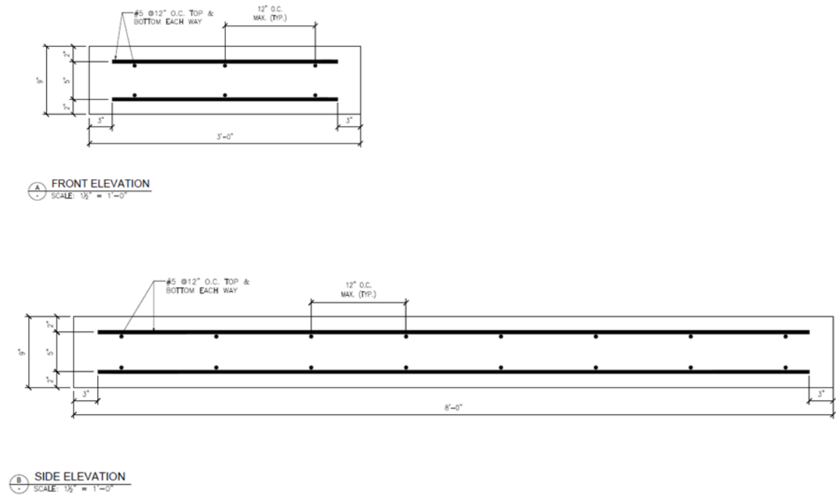
Figure 16. Details of the first specimen (Benchmark)
