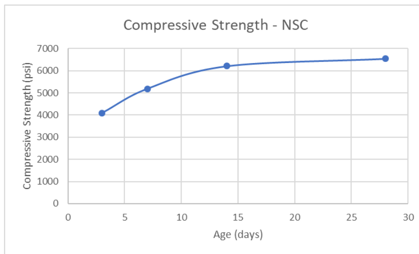
Figure 10. Compressive Strength Test Results, NSC
