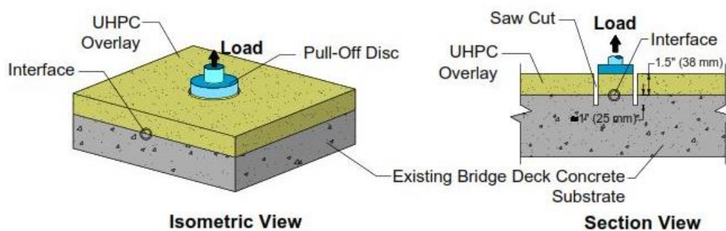
Figure 3. Illustration. Direct tension pull-off bond test based on ASTM C1583 [2].
