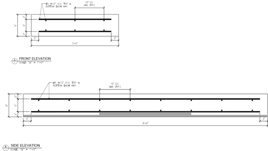
Figure 17. Details of the second specimen (bottom repair)
