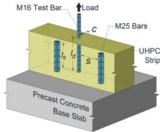
Figure 1 UHPC Connection Load Test Specimen Configuration (Graybeal, 2018)
