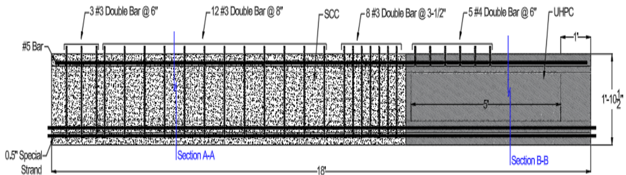
Figure 4. Elevation view of hybrid prestressed concrete girder specimen
