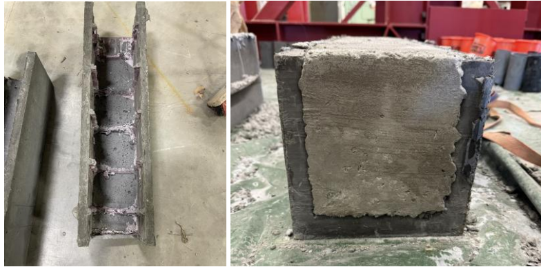
Figure 7. UHPC shell (left) and completed modulus of rupture specimen (right)
