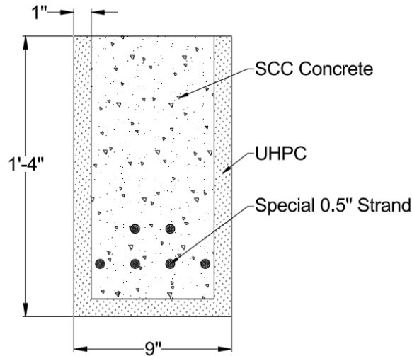
Figure 5. UHPC stay-in-place formwork specimen cross-section design
